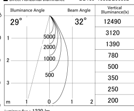
■ Direct Horizontal Illuminance DD139-1530DB9030D
