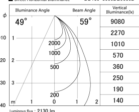
■ Direct Horizontal Illuminance DD139-3050DB9030D
