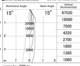
■ Direct Horizontal Illuminance DD139-3015DB9035D
