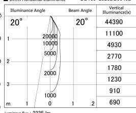
■ Direct Horizontal Illuminance DD139-2520DB9040D
