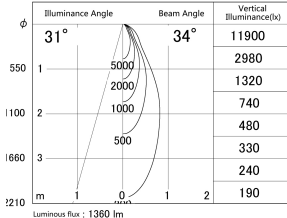
■ Direct Horizontal Illuminance DD139-1530WW9027D
