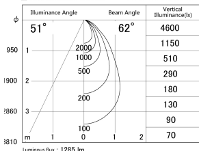
■ Direct Horizontal Illuminance DD139-1550WW9027D
