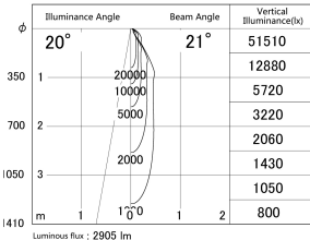
■ Direct Horizontal Illuminance DD139-3020WW9030D
