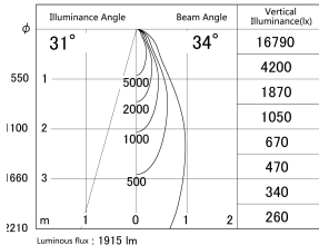
■ Direct Horizontal Illuminance DD139-2030WW9035D
