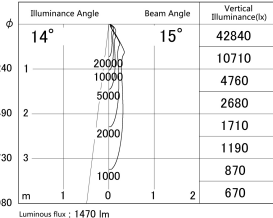
■ Direct Horizontal Illuminance DD139-1515WW9040D
