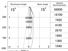
■ Direct Horizontal Illuminance DD139-3015WW9040D
