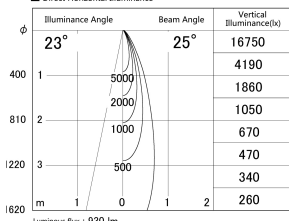
■ Direct Horizontal Illuminance DD161-1025MW9027
