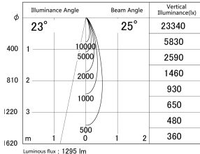
■ Direct Horizontal Illuminance DD161-1525MW9035
