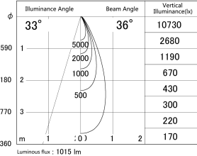
■ Direct Horizontal Illuminance DD161-1035MB9035
