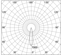
■ Direct Horizontal Illuminance DD161-0520MB9040
