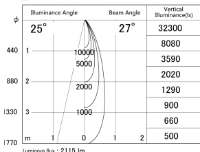
■ Direct Horizontal Illuminance DD161-2525MW9027-TL
