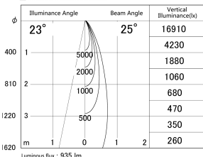
■ Direct Horizontal Illuminance DD161-1025MW9035-TL
