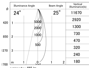
■ Direct Horizontal Illuminance DD161-0825MW9040-TL
