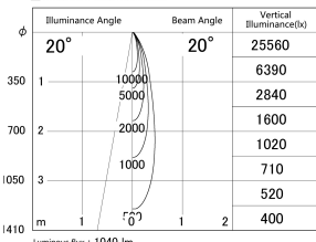
■ Direct Horizontal Illuminance DD161-1020MW9040-TL
