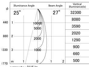
■ Direct Horizontal Illuminance DD161-2525MB9027-TL
