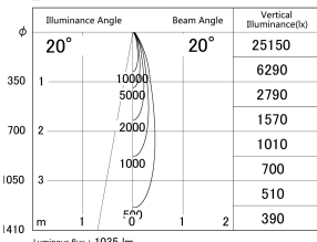
■ Direct Horizontal Illuminance DD161-1020WW9027-TL
