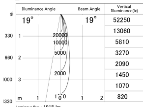
■ Direct Horizontal Illuminance DD161-2520WW9027-TL
