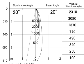
■ Direct Horizontal Illuminance DD161-0520WW9030-TL
