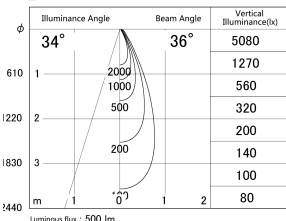
■ Direct Horizontal Illuminance DD161-0535WW9030-TL
