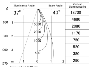
■ Direct Horizontal Illuminance DD161-2540WW9035-TL
