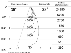
■ Direct Horizontal Illuminance (DD161-2540MB9040-FX)
