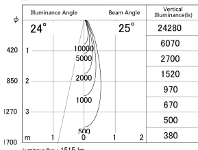
■ Direct Horizontal Illuminance DD161-1525WW9040-FX
