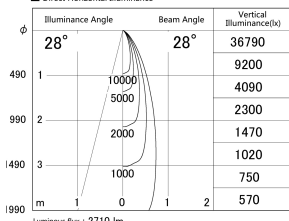
■ Direct Horizontal Illuminance (DD161-2525MB9027-FX-TL)
