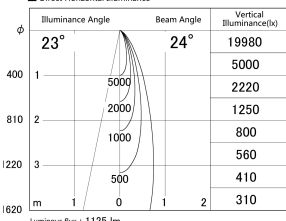
■ Direct Horizontal Illuminance (DD161-1025MB9030-FX-TL)
