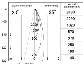
■ Direct Horizontal Illuminance (DD161-0525MB9035-FX-TL)
