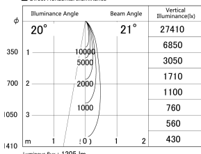
■ Direct Horizontal Illuminance (DD161-1020MB9040-FX-TL)
