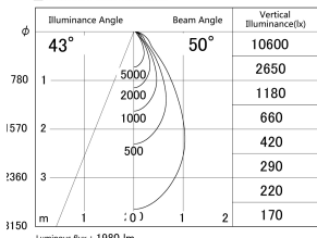
■ Direct Horizontal Illuminance DD161-2045WW9030-FX-TL
