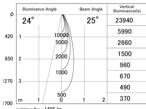
■ Direct Horizontal Illuminance DD161-1525WW9035-FX-TL
