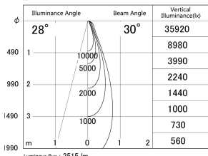
■ Direct Horizontal Illuminance DD146-2035W9030
