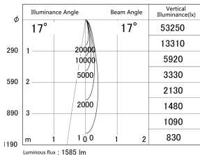
■ Direct Horizontal Illuminance DD155-1515MW9030-FX
