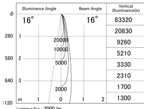
■ Direct Horizontal Illuminance DD155-2515DW9027-FX
