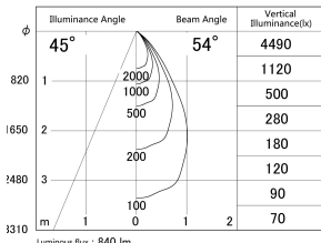
■ Direct Horizontal Illuminance DD155-0855DW9030-FX
