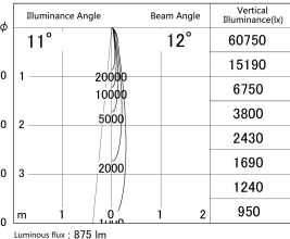
■ Direct Horizontal Illuminance DD155-1010MW9027
