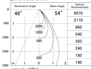
■ Direct Horizontal Illuminance DD155-1555MW9030
