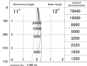
■ Direct Horizontal Illuminance DD155-1510DW9027
