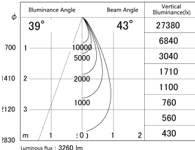
■ Direct Horizontal Illuminance DD155-3040DW9035
