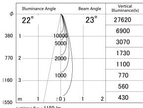
■ Direct Horizontal Illuminance DD155-1025DB9035
