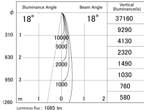
■ Direct Horizontal Illuminance DD155-1015DB9040
