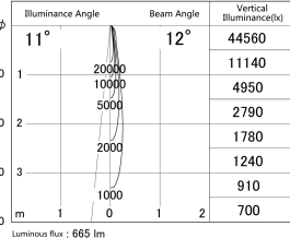
■ Direct Horizontal Illuminance DD155-0810WW9030
