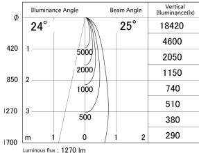
■ Direct Horizontal Illuminance DD133-1425W9027
