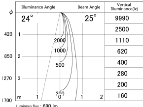
■ Direct Horizontal Illuminance DD133-0825W9027
