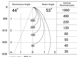
■ Direct Horizontal Illuminance DD133-0550W9027
