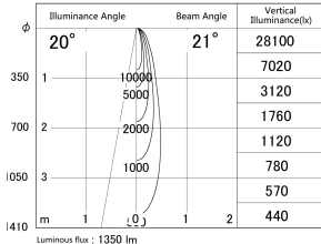
■ Direct Horizontal Illuminance DD133-1420W9030
