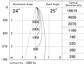
■ Direct Horizontal Illuminance DD133-1425W9030
