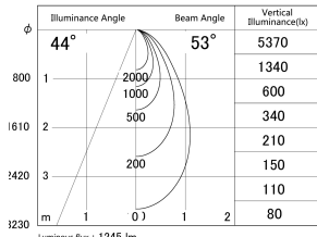
■ Direct Horizontal Illuminance DD133-1450W9030
