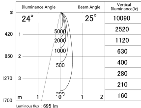
■ Direct Horizontal Illuminance DD133-0825W9030
